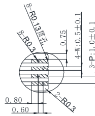
Detail A SCALE 3:1
